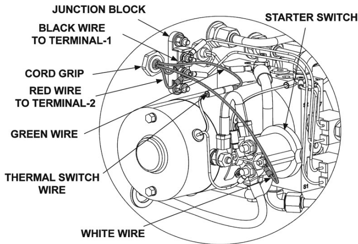
CONTROL SWITCH WIRING CONNECTIONS FIG. 37-2
